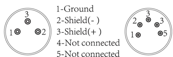
XLR mounting-plugs
