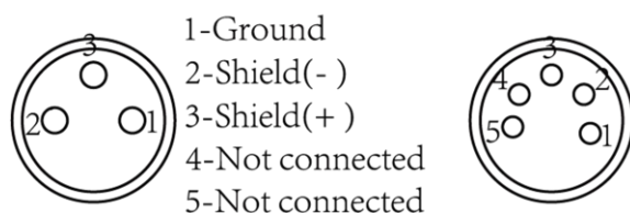
XLR mounting-sockets
